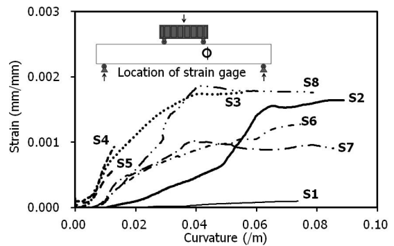
Fig. 10 Strains of Tie Bars
