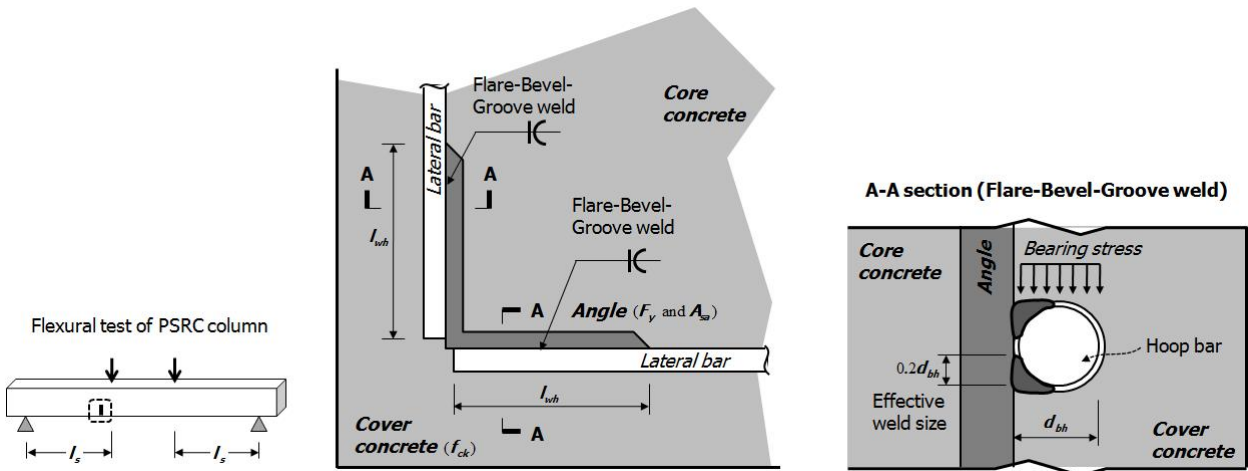
Fig. 4 Bond strength between angle and concrete of PSRC member
