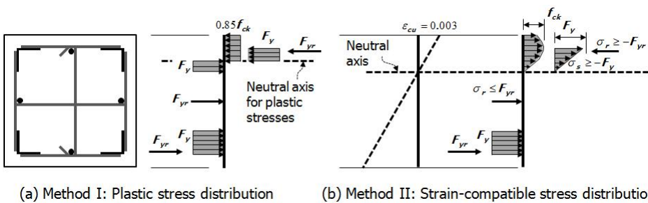
Fig. 2 Flexural strength of PSRC member
