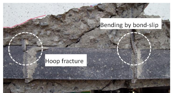
Fig. 12 Dowel Action and Fracture of Lateral Re-bars After Bond Failure Between Angle and Concrete
