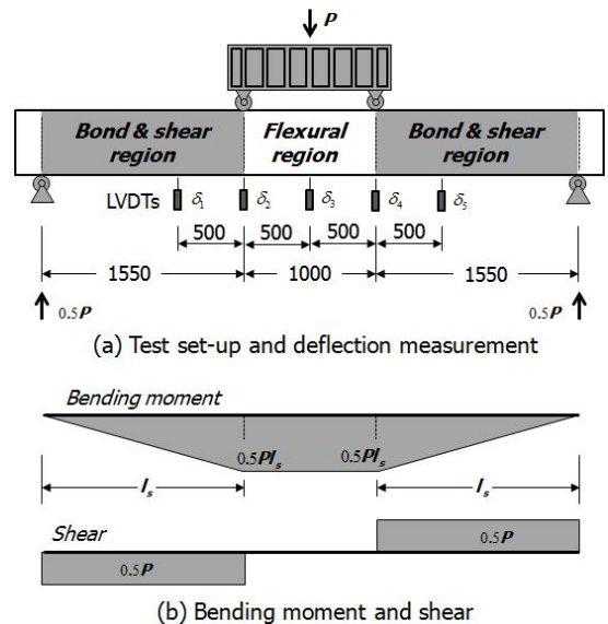
Fig. 6 Test Set-up for Loading and Measurement
