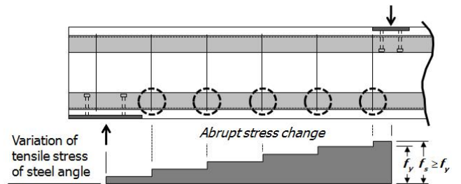
Fig. 11 Stress Concentration at Weld Joints Between Angle and Lateral Re-bars
