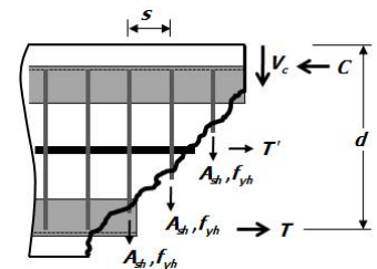
Fig. 3 Shear strength
