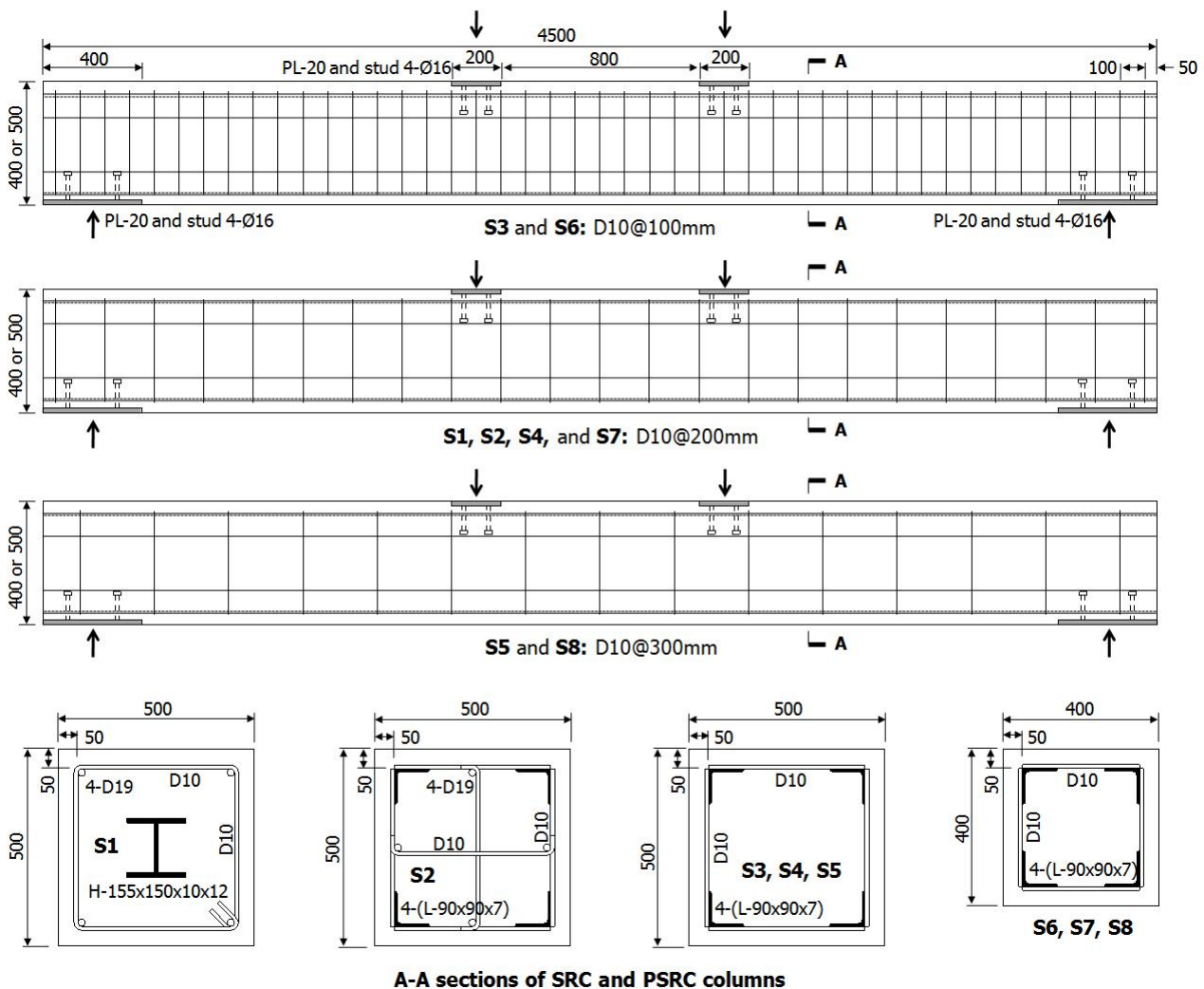
Fig. 5 Geometric Properties of Test Specimens
