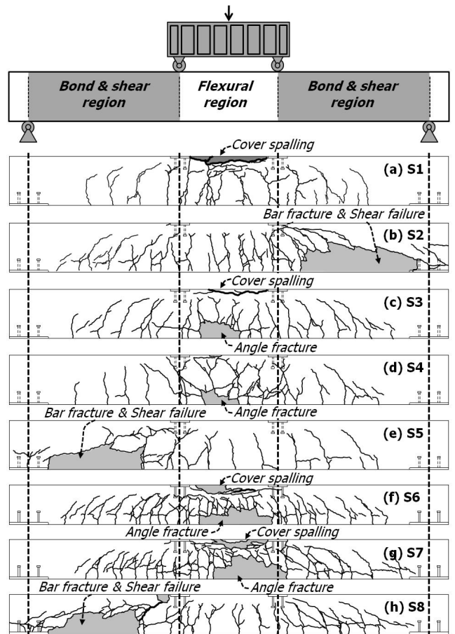
Fig. 8 Failure Modes of Specimens
