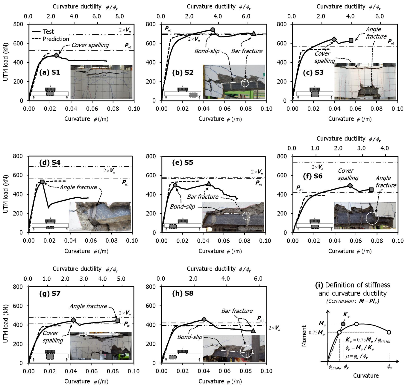
Fig. 7 Moment-curvature Relationships at the Center Span of Specimens
