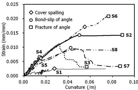
Fig. 9 Longitudinal Strains of Steel Sections
