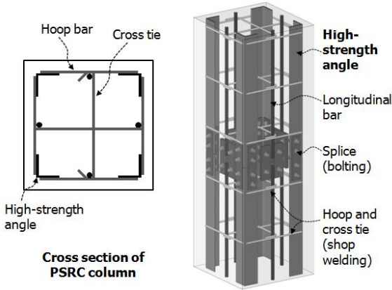
Fig. 1 Composite columns using steel angles
