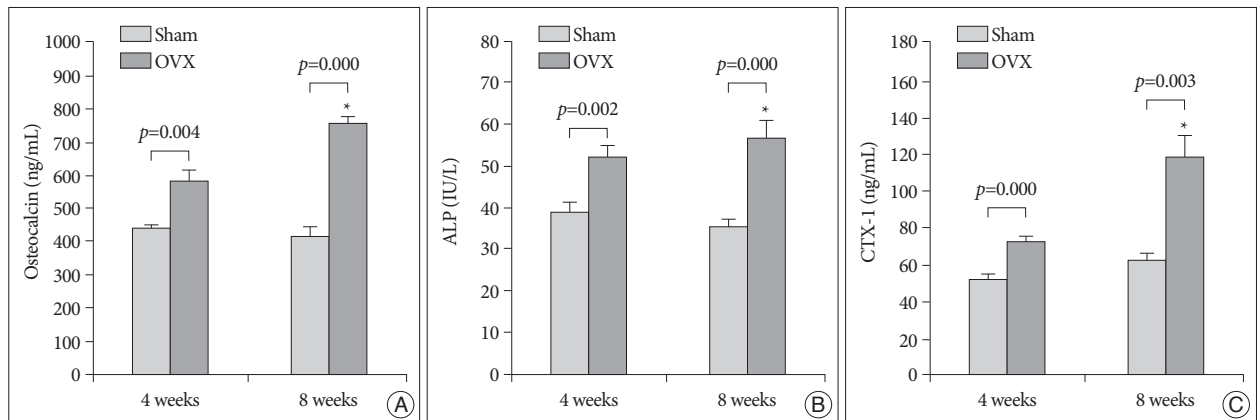
Fig. 3. The serum osteocalcin (A) and ALP (B) concentrations were used as markers of bone formation. Type I collagen C-telopeptide (CTX) (C) concentration was used as a marker of bone resorption. Values are mean \pm standard deviations. *indicates p < 0.05 for 4 weeks vs. 8 weeks in the OVX group. ALP : alkaline phosphatase, OVX : ovariectomized.
