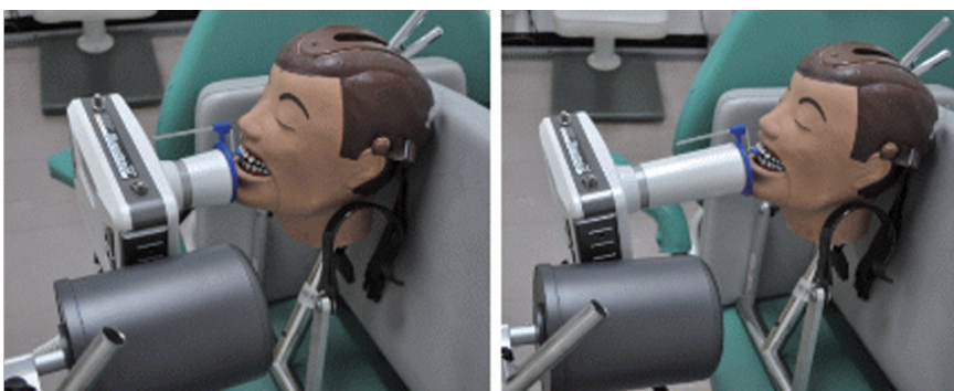
Figure 8. Operator's radiation dose at hand level of operator was measured using short and long cones.
