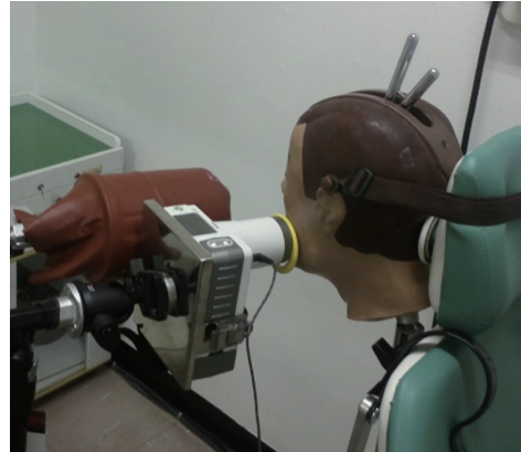
Figure 7. Radiation doses were measured at the hand level of operators using an ionization chamber covered with a lead sleeve.
