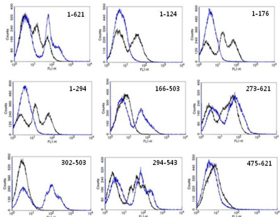
Figure 8. Domain-level epitope mapping of ER2 using the yeast surface-expressed EGFR fragments. Representative flow cytometry histograms depict anti-c-myc 9e10 labeling for the expression of EGFR fragments (black) and ER2 binding (blue) to the yeast surface-expressed EGFR fragments, as indicated in each panel. For the whole EGFR (1~621), the 404SG mutant was used (described in detail in the text).
