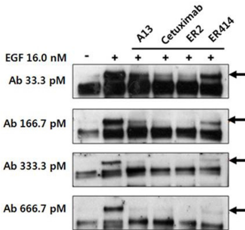
Figure 7. Blocking of the EGF-induced tyrosine phosphorylation of EGFR by A13 mAb, ER414, ER2 and cetuximab in MDA-MB-231 cells. The serum-starved cells were untreated, treated with EGF (16 nM) only, or treated with EGF (16 nM) and 33.3, 166.7, 333.3 or 666.7 pM of mAbs for 30 min, as indicated in the panels, before the Western blotting analyses. The arrows indicate the expected size (~170 kDa) of the EGFR.
