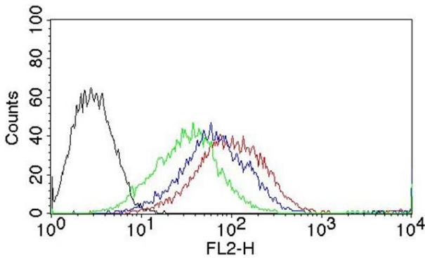
Figure 6. Binding of anti-EGFR mAbs to cell surface-expressed EGFR. Differential binding of mAbs to EGFR-positive A431 tumor cells was determined by flow cytometry. Histograms in different colors represent the reactions of labeled secondary Ab with A431 cells (black), ER414 with A431 cells (green), ER2 with A431 cells (blue), and mAb A13 with A431 cells (red).
