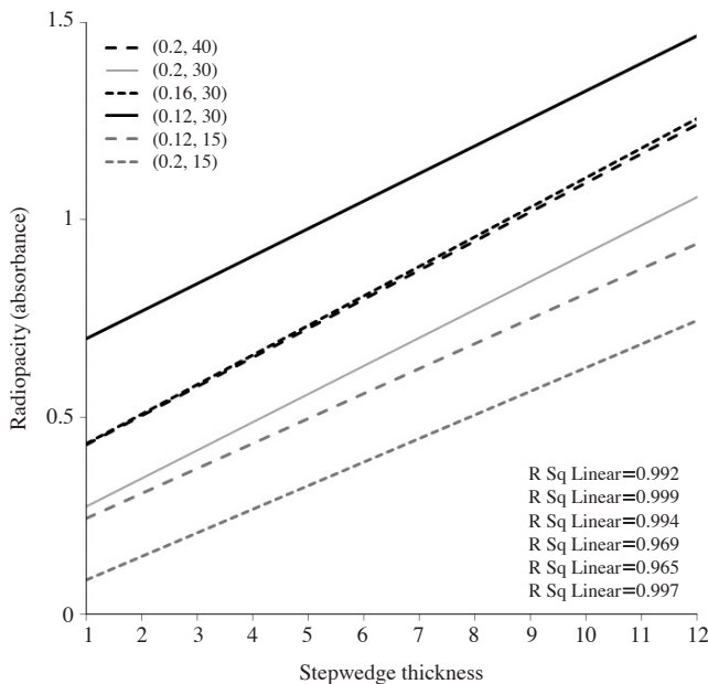
Fig. 1. Linear models with corresponding R^2 obtained from various distance/exposure time setups for aluminum step wedge.
