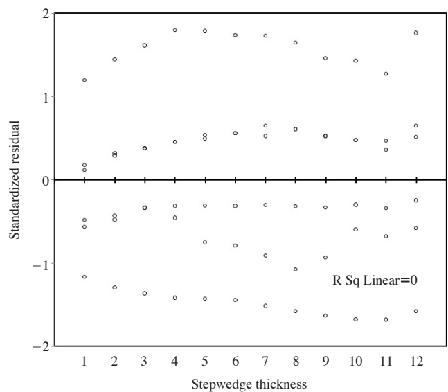
Fig. 2. Magnitude of residue for corresponding thickness of aluminum stepwedge.
