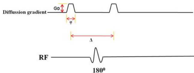
Fig. 3. (Color online) The length of the gradient pulses is denoted by \delta with an amplitude equal to G_D . The space in between them, the diffusion time, is denoted by \Delta . By employing a 180^\circ RF, dephasing from T_2^* is reduced causing an increase in signal for data collection.
