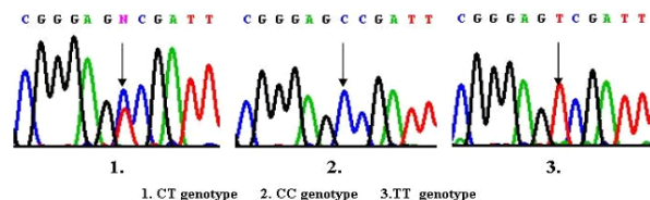
Figure 2. The Sequencing of MTHFR C677T Site Digested by Hinf I (Points to SNP)
