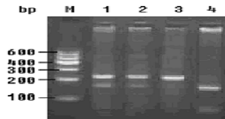
MI : 100bp ladder; 1 and 2 :CT; 3: CC; 4: TT; Figure 1. Electrophoresis Chart of PCR Products Containing Site C677T of MTHFR Digested by Hinf I
