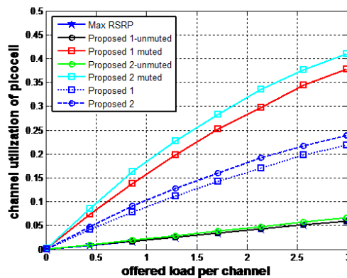
Fig. 7. Channel utilization in each picocell
