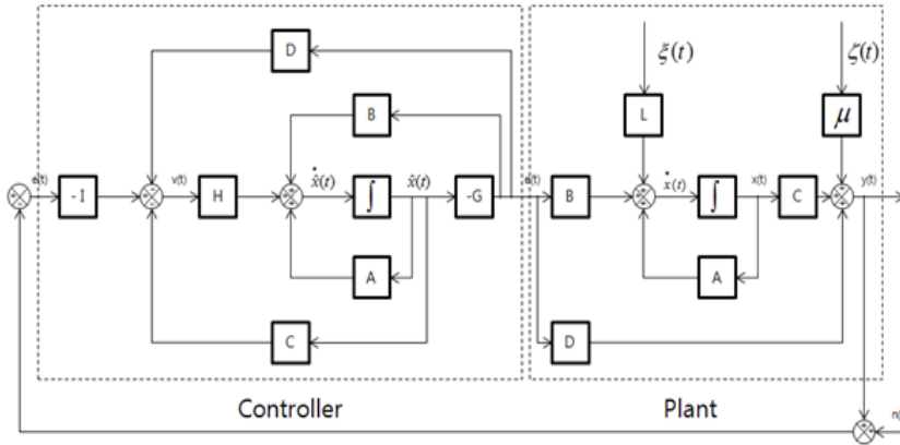
Fig. 5 Structure of the LQG/LTR controller
