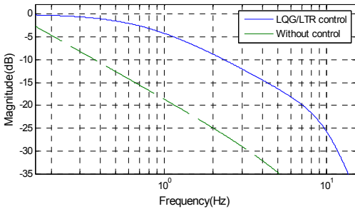
Fig. 8 FRF of identified system without control and simulated FRF of closed loop system
