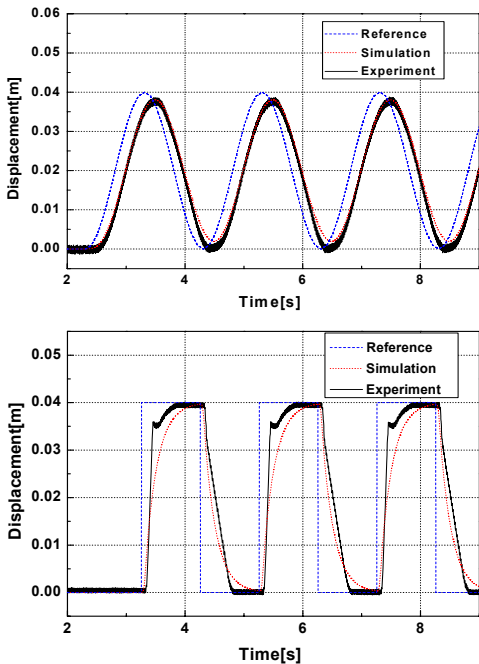
Fig. 13 Responses of the closed loop control system with dead-zone compensator to 0.5 Hz sine and square input
