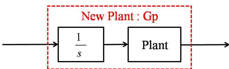
Fig. 4 New plant combined with an integrator
