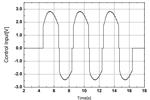
Fig. 11 Response of the closed loop control system with dead-zone compensator to 0.25 Hz sine input and control input
