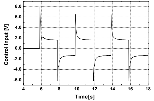
Fig. 10 Response of the closed loop control system without dead-zone compensator to square input and control input
