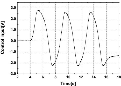
Fig. 9 Response of the closed loop control system without dead-zone compensator to sine input and control input
