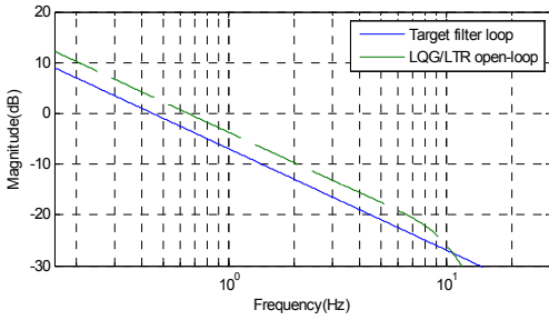
Fig. 7 FRF of the target filter loop and the open loop system
