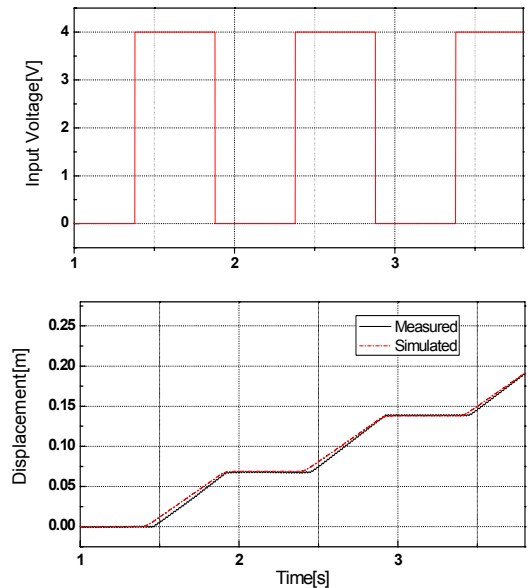
Fig. 3 Comparison of measured and simulated system response
