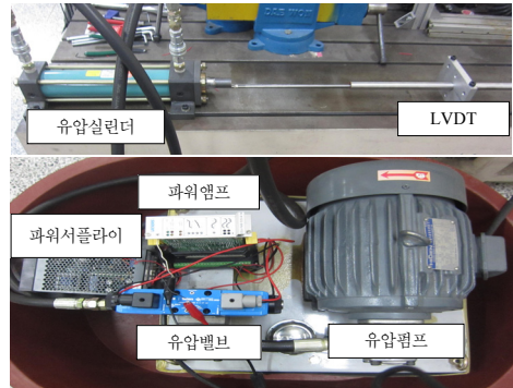
Fig. 1 Experimental equipment
