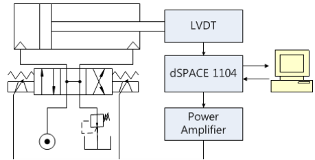
Fig. 2 Schematic diagram of experimental device
