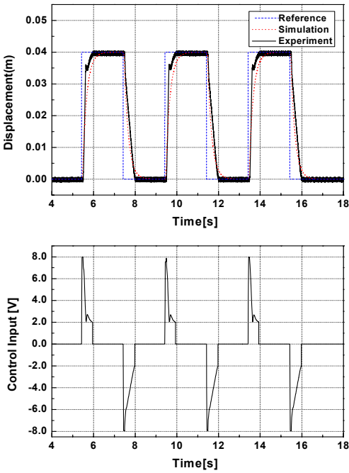
Fig. 12 Response of the closed loop control system with dead-zone compensator to square input and control input
