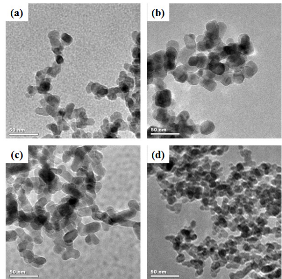
Fig. 6. TEM images of SnO 2 nanoparticles synthesized using various solvents; (a) deionized water, (b) methanol, (c) ethanol, (d) propanol.
