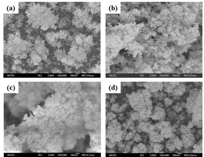
Fig. 5. FE-SEM images of SnO 2 nanoparticles synthesized using various solvents; (a) deionized water, (b) methanol, (c) ethanol, (d) propanol.
