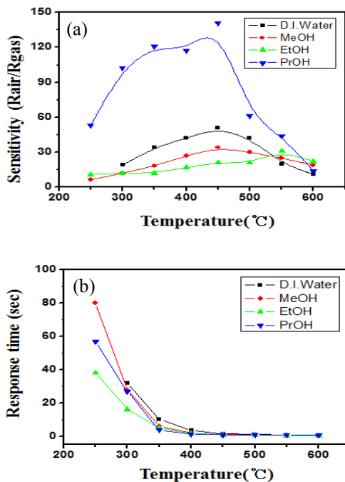
Fig. 7. Sensing properties of SnO 2 nanoparticles synthesized in various solvents toward 1,000 ppm H 2 gas as a function of operating temperature.
