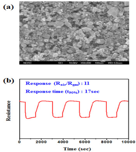
Fig. 4. (a) FE-SEM image of commercial SnO 2 nanopowder, (b) Response transient of commercial SnO 2 toward H 2 1,000 ppm gas.
