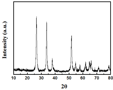
Fig. 1. X-ray diffraction patterns of the SnO 2 nanoparticles synthesized by flame spray pyrolysis using aqueous solution.
