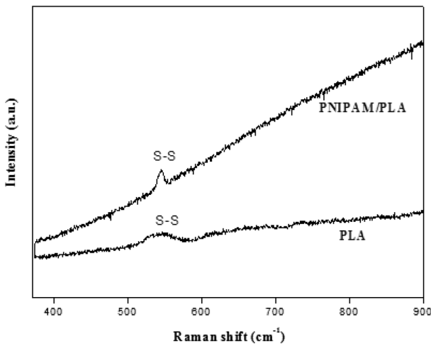
Figure 2. Raman spectra of PLA and PNIPAM/PLA10 hydrogels.
