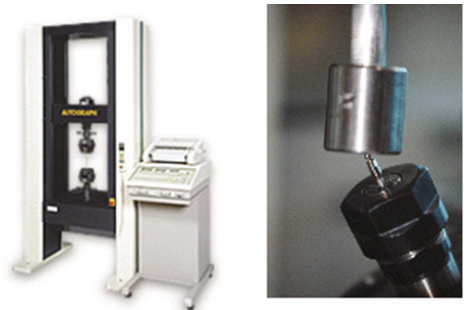
Fig. 3. Universal testing machine for static loading test (AGS-1000D, SHIMADZU Co., Japan).
