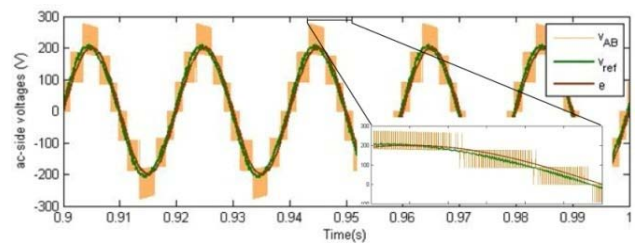
Fig. 5. Grid and ac-side voltage of the CHB inverter during the first simulation.
