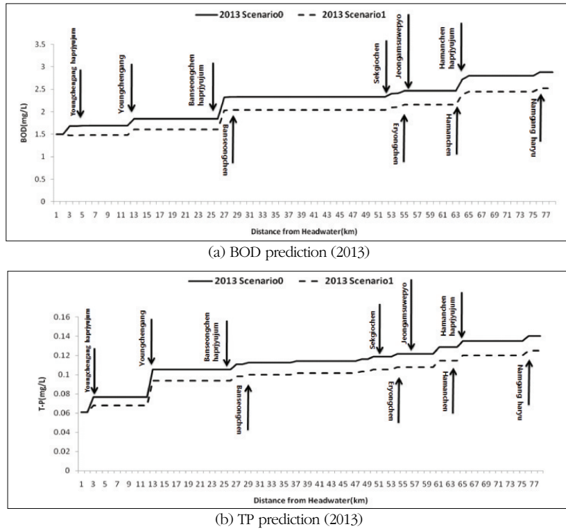
Fig. 7. Results of BOD and TP prediction with QUALKO2 in Milyanggang mid-watershed
