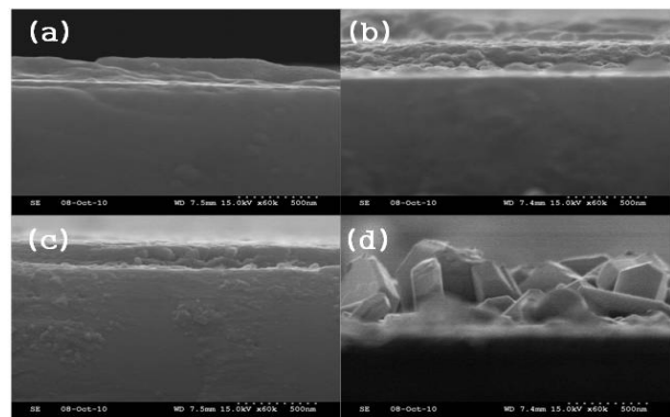
Fig. 4. Cross-section image of AZO (Al-doped zinc oxide) thin film at (a) RT, (b) 400°C, (c) 500°C, and (d) 700°C.
