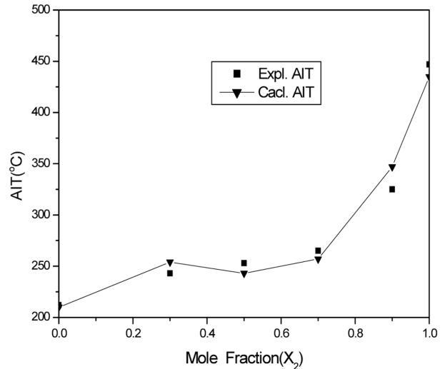
Figure 1. Comparison of AIT prediction curves with experimental data for n-decane(X 1 )+sec-butanol(X 2 ) system.
