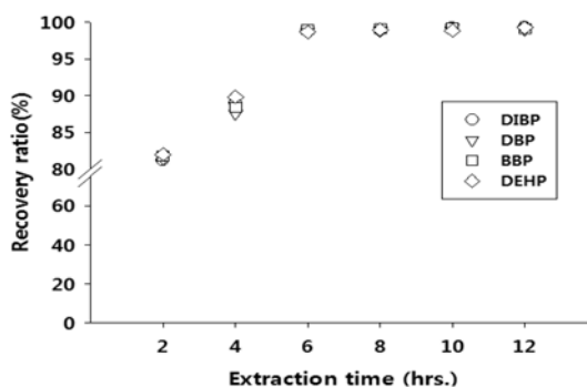
Fig. 3. Recovery ratios of phthalates from EPDM rubber using hexane according to different Soxhlet-extraction times.
