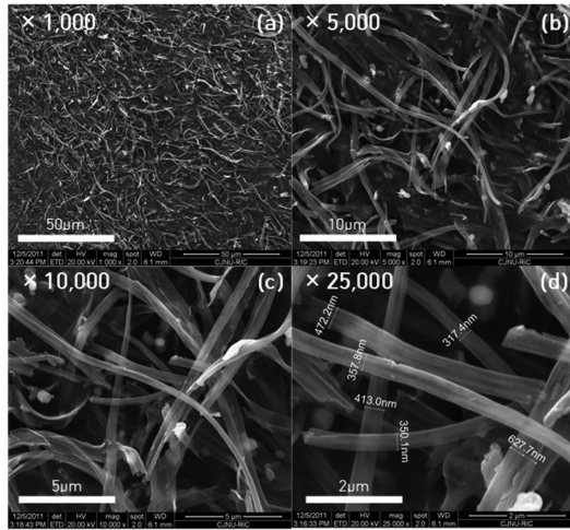
Fig 2. SEM image of \text{Li}[\text{Fe}_{0.9}\text{Mn}_{0.1}]\text{PO}_4 nano-fibers. ; (a) \times 1,000 , (b) \times 5,000 , (c) \times 10,000 , (d) \times 25,000 .
