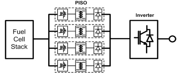
Fig. 2. The PISO system with fuel cell of LoV-HiC.
