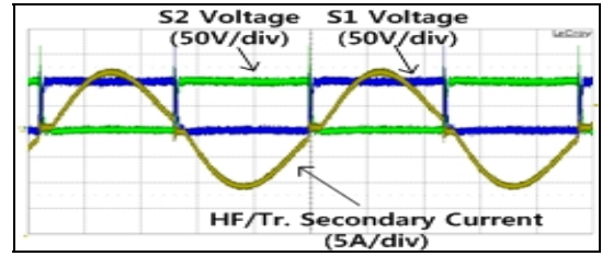
(a) Switch voltage and transformer secondary current
