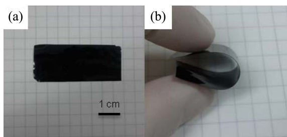
Figure 2. Photographic images of the free (a) and bent (b) 6TTF-polymer films.
