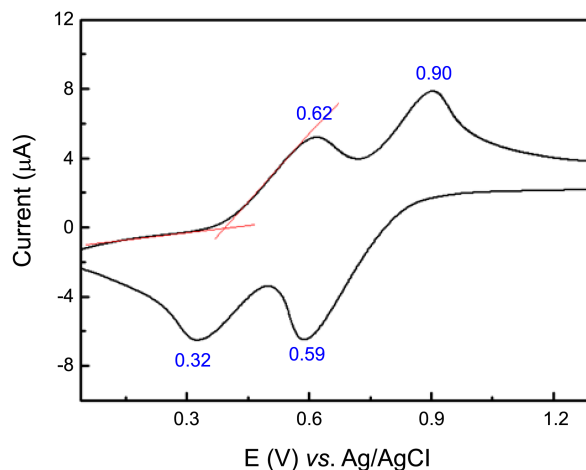
Figure 3. Cyclic voltammogram of the 6TTF-polymer (0.01 mM in \text{CH}_2\text{Cl}_2 ). Here, \text{Bu}_4\text{ClO}_4 (0.1 M) worked for a supporting electrolyte. A glass carbon electrode, an Ag/AgCl electrode and a platinum wire were also used as a working electrode, a reference electrode and a counter electrode, respectively.
