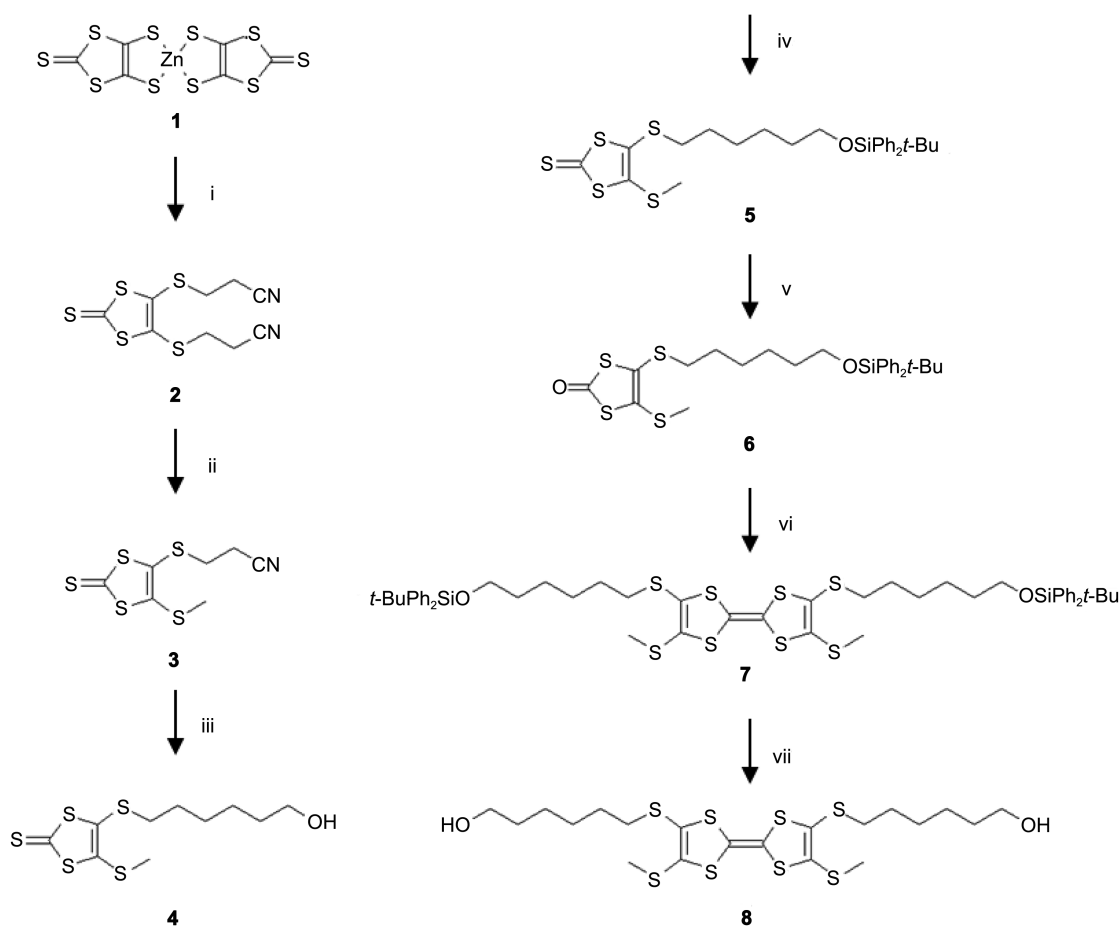
Scheme 1. Reagents and conditions: (i) \text{Br}(\text{CH}_2)_2\text{CN} , acetone, reflux, overnight; (ii) \text{CsOH}\cdot\text{H}_2\text{O} , dimethylformamide, methanol, iodomethane, 20\text{ }^\circ\text{C} \rightarrow 60\text{ }^\circ\text{C} ; (iii) \text{CsOH}\cdot\text{H}_2\text{O} , methanol, then, \text{Br}(\text{CH}_2)_6\text{OH} , 20\text{ }^\circ\text{C} , 12 h; (iv) t\text{-BuPh}_2\text{SiCl} , imidazole, N,N -dimethylformamide, 20\text{ }^\circ\text{C} ; (v) \text{Hg}(\text{OAc})_2 , 0.5 h; (vi) \text{P}(\text{OEt})_3 , 130\text{ }^\circ\text{C} , 3 h; (vii) TBAF in THF, tetrahydrofuran, 20\text{ }^\circ\text{C} , 24 h.
