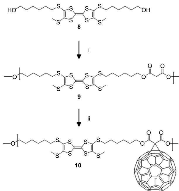
Scheme 2. Reagents and conditions: (i) malonyl chloride, triethylamine, dichloromethane; (ii) DBU, tetrabromomethane, toluene, 70\text{ }^\circ\text{C} , 40 h.
