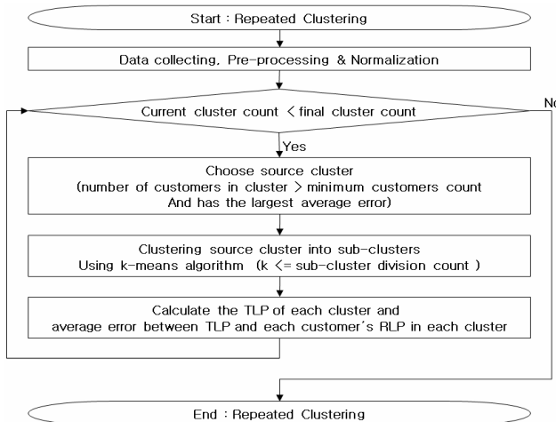
Fig. 4. Flow diagram of repeated clustering
