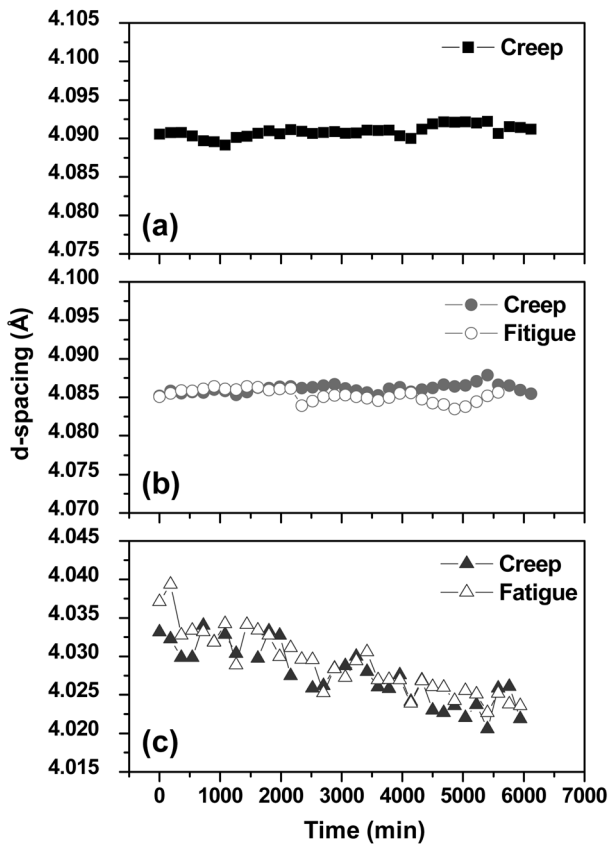
Figure 7. Change of d -spacing of (110) plane during creep and fatigue tests for BYP (a); YP (b); AYP specimen (c).
