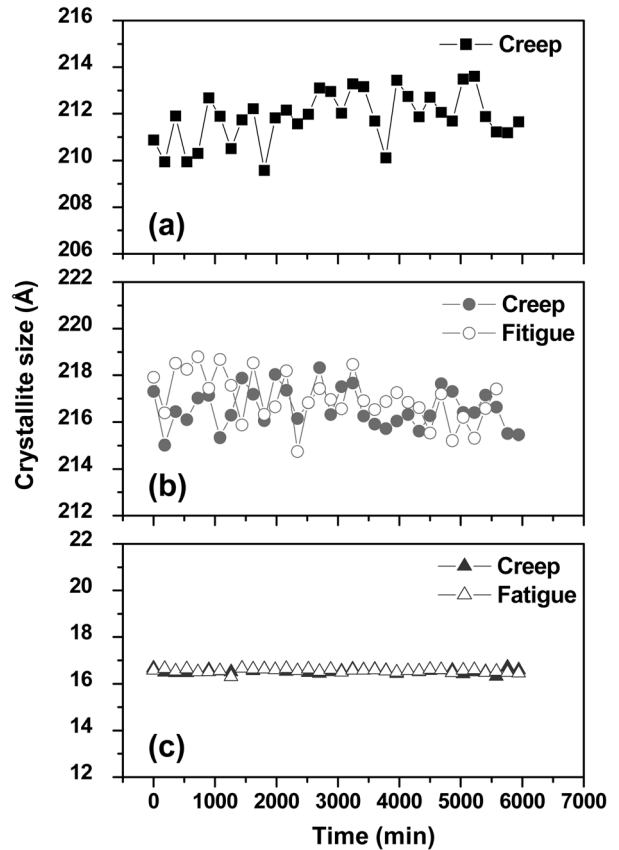
Figure 6. Change of crystal size of (110) plane during creep and fatigue tests for BYP (a); YP (b); AYP specimen (c).
