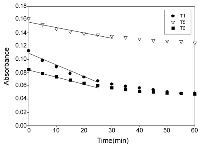
Figure 7. Color-fading speed of coating films prepared with different organic contents after UV irradiation.
