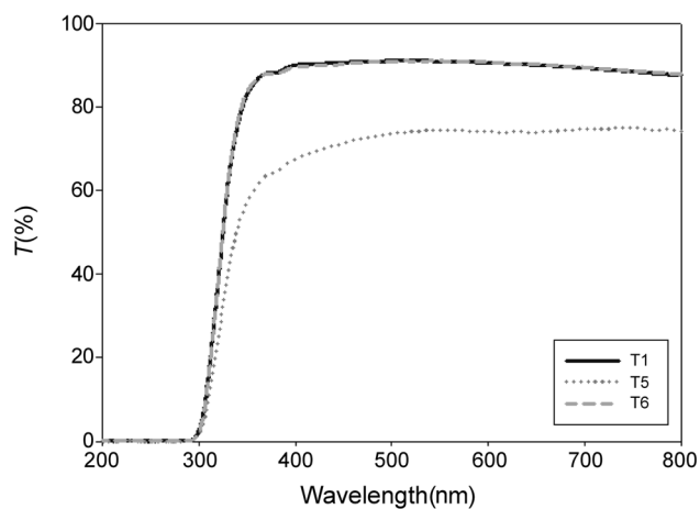
Figure 8. Transmittance of coating films prepared with different organic contents before UV irradiation.
