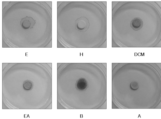
Fig. 3. Fibrinolytic activity of SA by fibrin-plate assay E, 70% Ethanol extract; H, Hexane fraction; DCM, Dichloromethane fraction; EA, Ethyl acetate fraction; B, Butanol fraction; A, Aqueous fraction.
