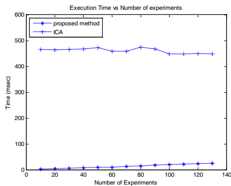
Fig. 5. Plot of execution time against number of experiments in microarray data.
