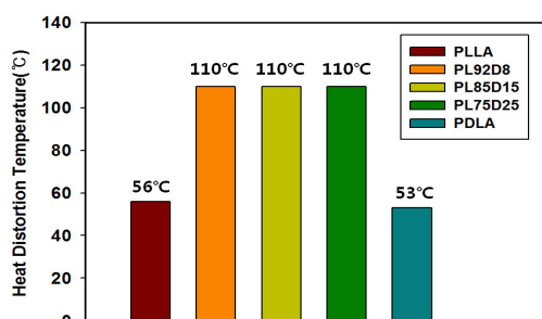
[Fig. 3] Heat distortion temperatures of PLA SC blends
