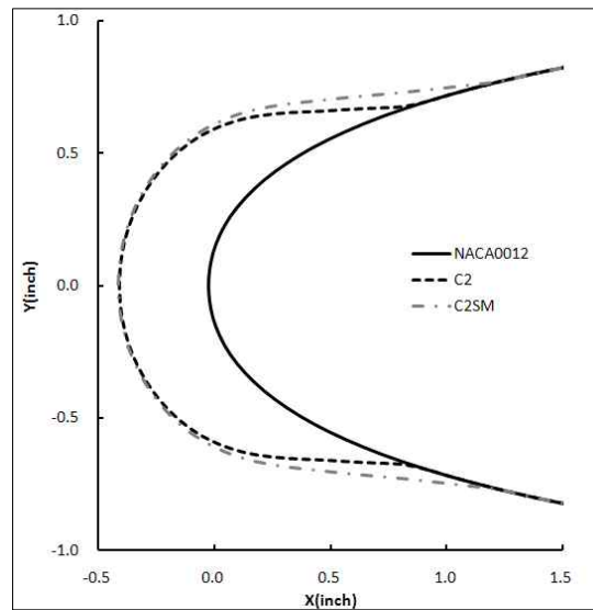
Fig. 4. Comparison of ice shapes after scaling (stratiform C2)
