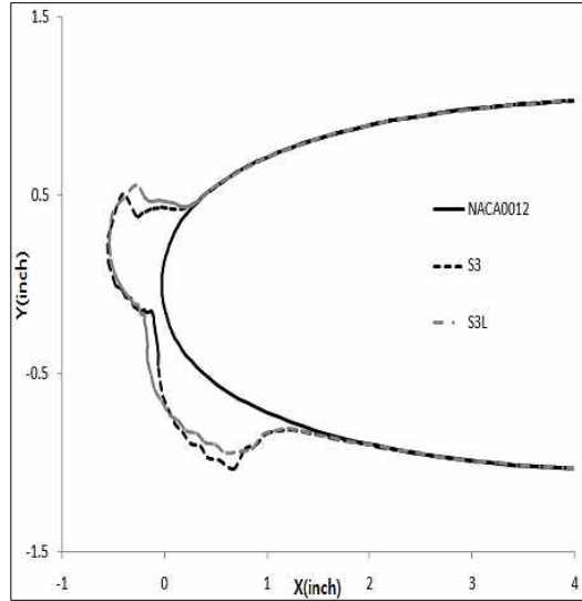
Fig. 7. Comparison of ice shapes after scaling (horn)
