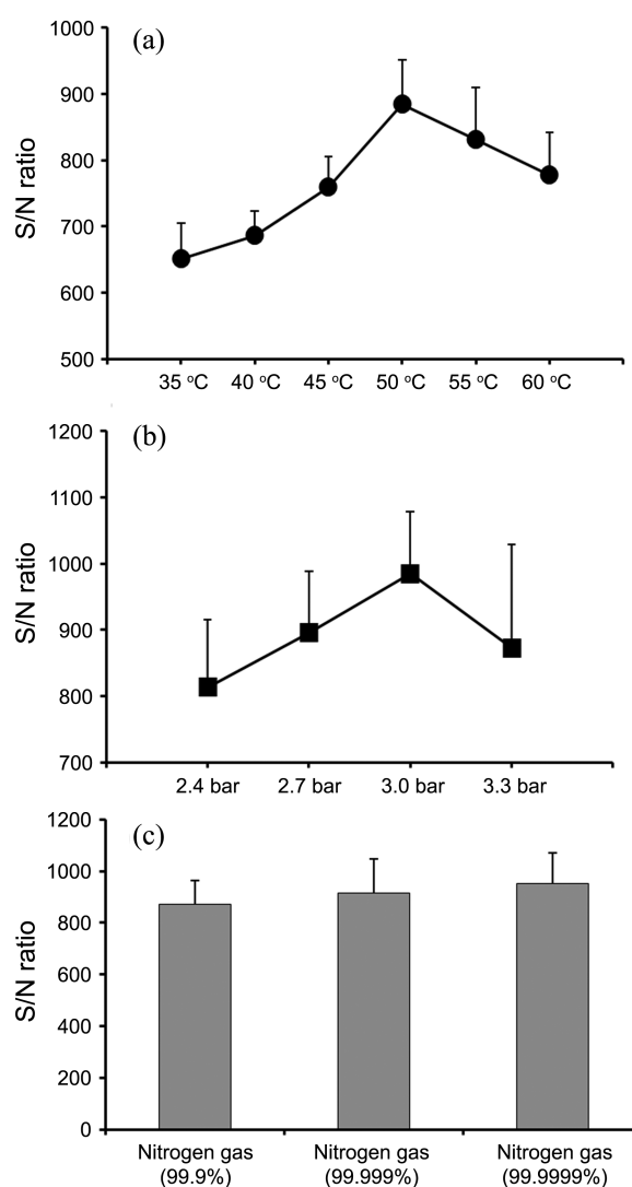
Figure 4. Optimization of the ELSD parameters. Drift tube temperature (a), nebulizing gas (N 2 ) pressure (b), and nitrogen gas purity (c).
