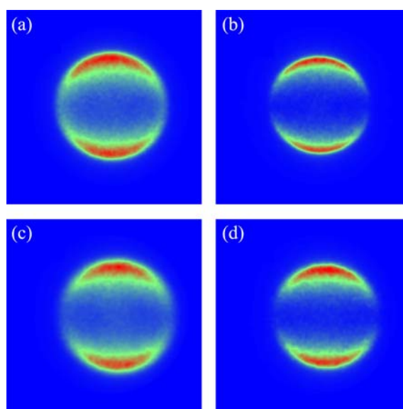
Figure 1. Raw ion images of (a) Br and (b) \text{Br}^* from the photodissociation of \text{C}_3\text{H}_5\text{Br} . Those of Br and \text{Br}^* from \text{C}_4\text{H}_7\text{Br} are shown in (c) and (d), respectively. In all images, the polarization vector of the photolysis laser is vertical.
