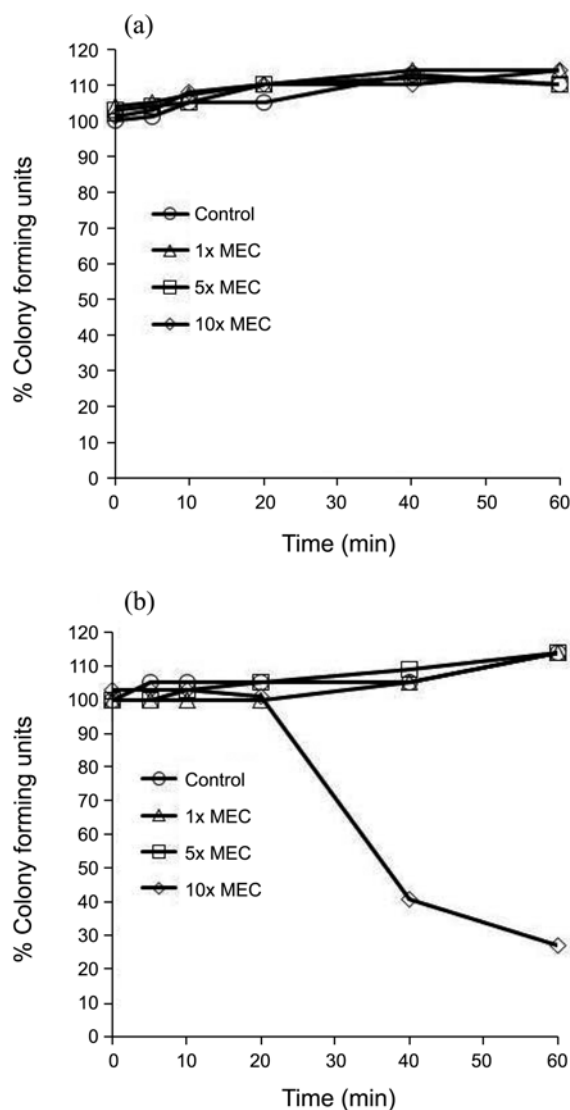
Figure 2. Bacterial killing kinetics of apidaecin Ib (a) and gentamicin (b) at different time intervals against E. tarda H-4: Control (without antimicrobial agents, O), 1×MEC ( \Delta ), 5×MEC ( \square ), and 10×MEC ( \diamond ).
