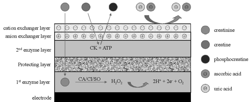
Fig. 2. The concept of an amperometric creatinine biosensor with reduced interference from creatine: CK, creatine kinase; ATP, adenosine triphosphate; CA, creatinase; CI, creatinase; SO, sarcosine oxidase.
