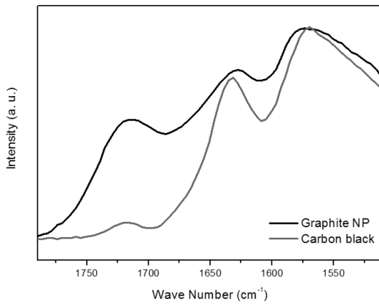
Fig. 3. FT-IR spectrum for graphite nanoparticles prepared by liquid phase pulse laser ablation and commercial carbon black.
