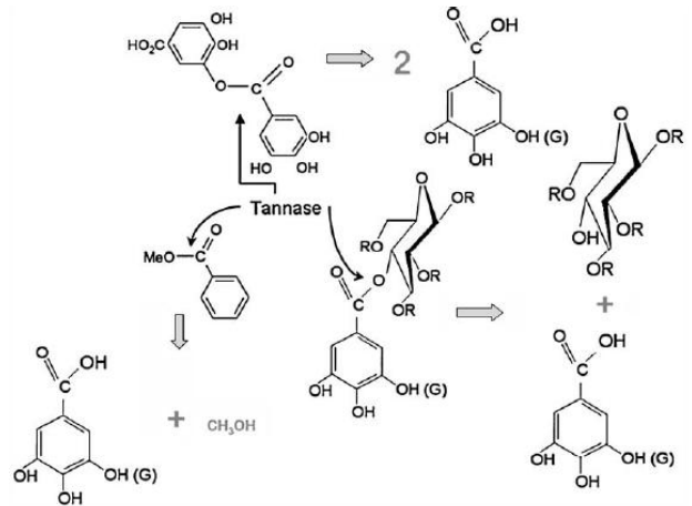
Fig. 3. Gallic acid production mechanism of active of tannase.
