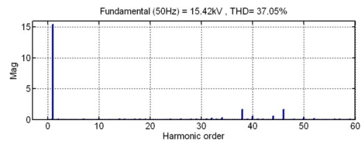
(c) Line voltage spectrum.
