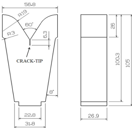
Fig. 1 Geometry and dimensions of specimen (unit : mm)
