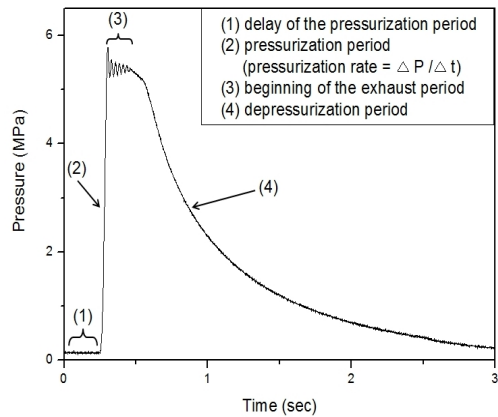
Fig. 4 Typical pressure-time trace of the experiment
