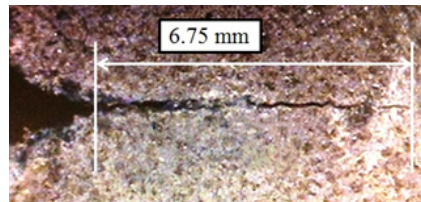
(a) 64.34 MPa/s
