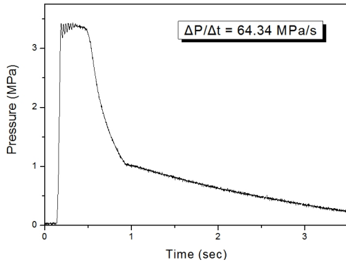
(a) 64.34 MPa/s
