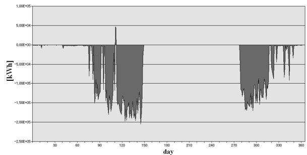
Fig. 16. Detailed variation of electricity production due to thermal networking operation on the existing DHC system side
