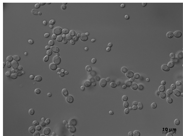
Fig. 1. Microscopic features of Pichia farinosa NAAS-2 (× 1000).
