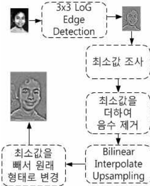
Fig. 4. Reconstruction process of edge map
