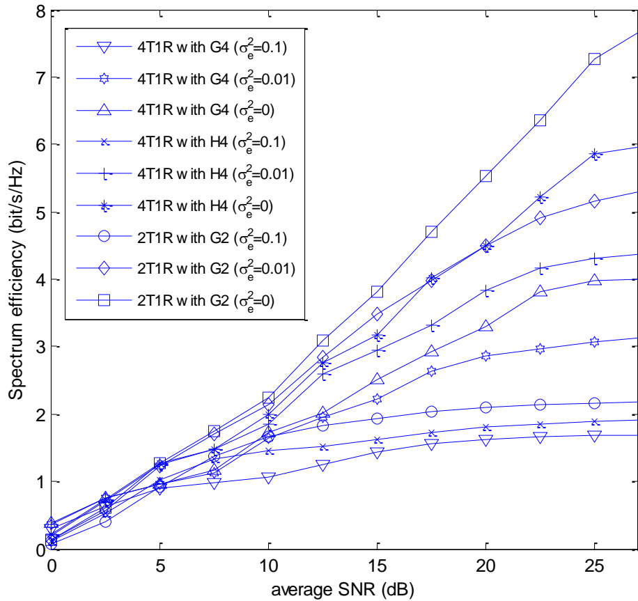
Fig. 4. SE of AM-STBC with different transmit antennas and one receive antenna for different estimation errors under imperfect CSI. ( K=3 dB)
