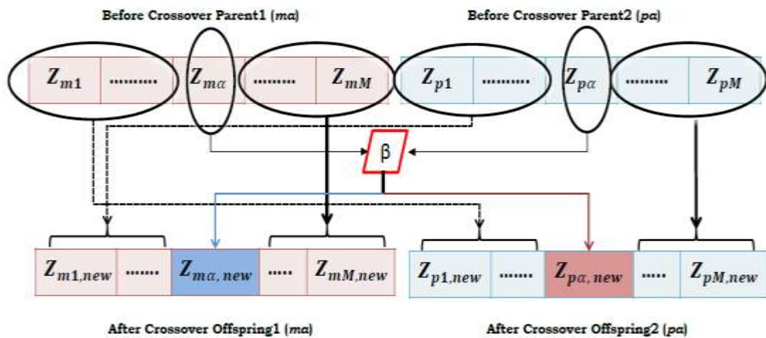
Fig. 2. GA crossover operation
