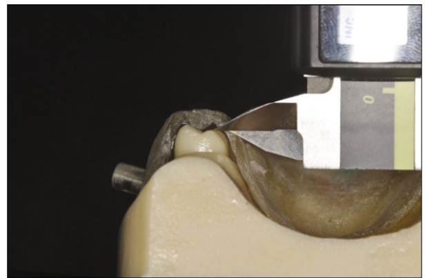
Fig. 7. Measuring the gap between the surgical guide and the model to evaluate the fitness.
