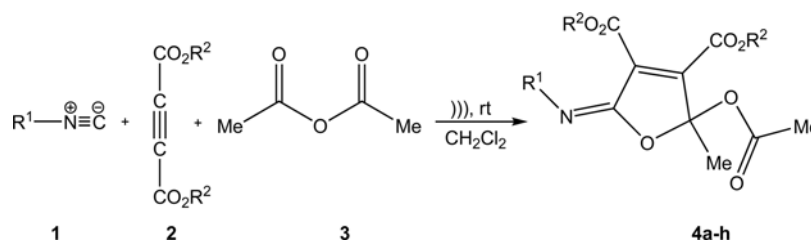
Scheme 1. Three-component synthesis of 2,5-dihydro-5-imino-2-methylfuran-3,4-dicarboxylate derivatives 4 under ultrasound irradiation (see Table 1).
