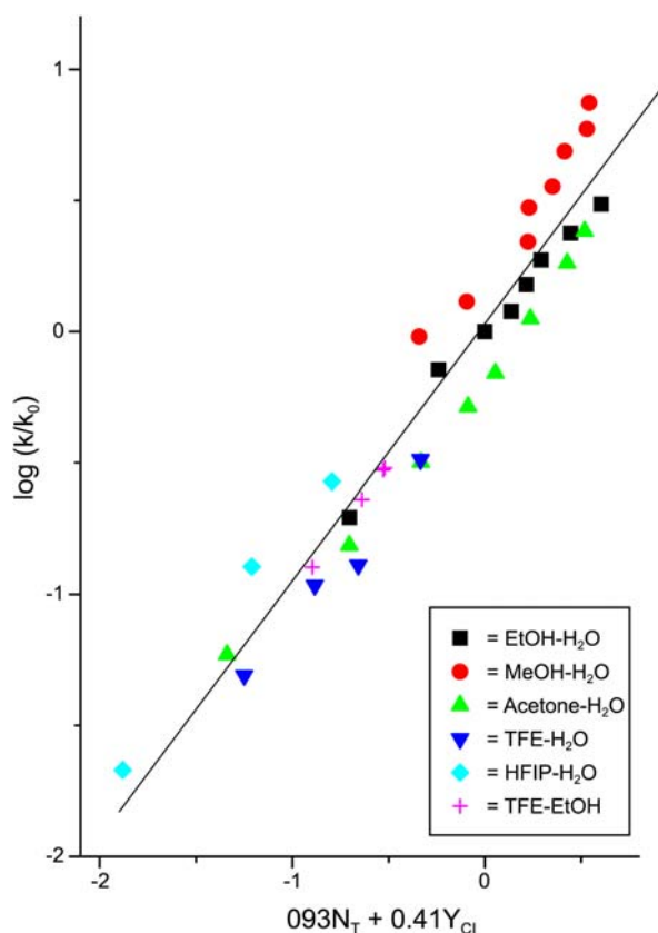
Figure 1. Plots of \log(k/k_0) for the solvolysis of allyl chloroformate ( 3 ) at 35.0 °C against (0.93 N_T + 0.41 Y_{Cl}) .
