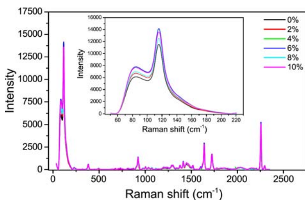
Figure 4. Raman spectra for DSSCs made with a liquid electrolyte and UV-cured resin electrolytes with different GBL concentrations. The inserted is the Raman spectra of the region of the I_3^- species.
