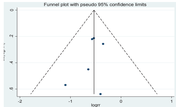
Figure 3. Funnel Plot for Assessing Publication bias in this Meta-analysis
