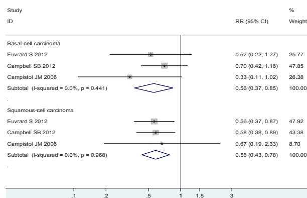
Figure 2. Forest Plot for the Meta-analysis of Sirolimus in Non-melanoma Skin Cancer Prevention by Histological Type
