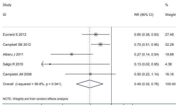
Figure 1. Forest Plot for the Meta-analysis of Sirolimus in Non-melanoma Skin Cancer Prevention
