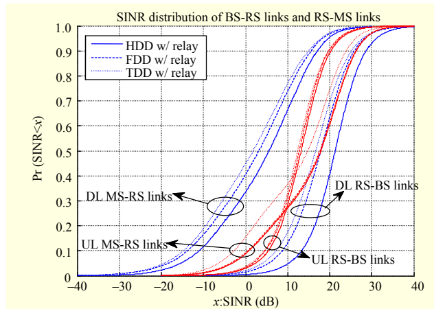
Fig. 6. SINR distribution of proposed, FDD, and TDD systems.
