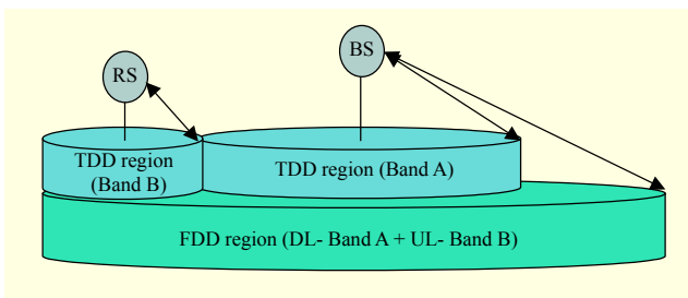
Fig. 1. Overlaid HDD system.
