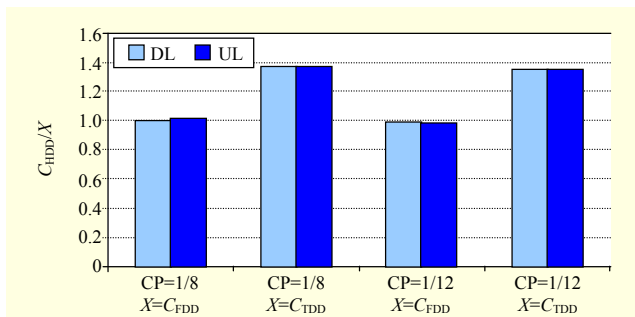
Fig. 4. Ratio between C_{HDD} and C_{FDD} (or C_{TDD} ).
