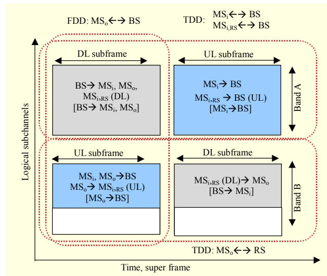
Fig. 2. Frame structure of overlaid HDD system.
