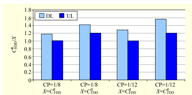
Fig. 5. Ratio between C_{HDD}^R and C_{FDD}^R (or C_{TDD}^R ).
