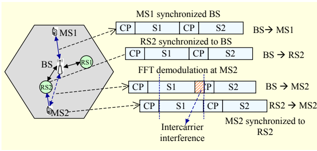
Fig. 3. OFDMA ICI with multiple sources and destination.
