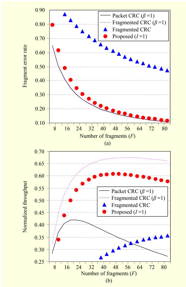
Fig. 6. Fragment error and throughput of each framing scheme at \alpha=1-10^{-3} , \beta=1 and 1-10^{-6} .
