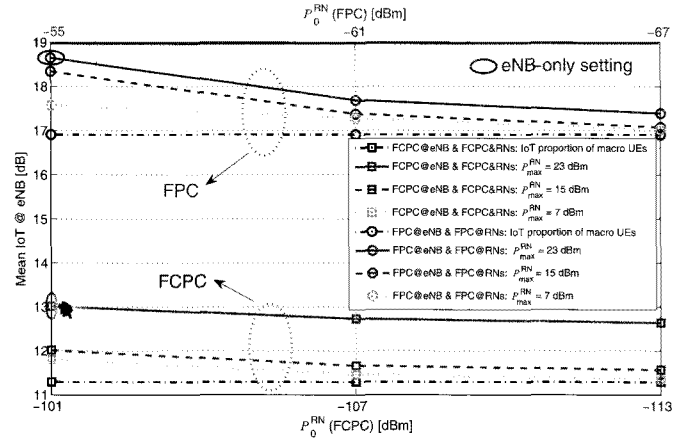
Fig. 6. Mean IoT at eNB vs. P_0^{RN} for different P_{max}^{RN} values. The simulation results are given for FPC and FCPC settings. eNB-only settings are denoted by ellipses.
