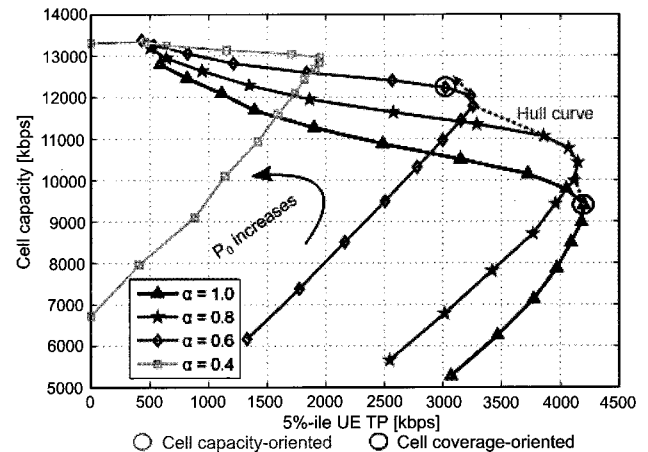
Fig. 4. Cell capacity vs. 5%-ile user TP for different values of \alpha in eNB-only deployment. The hull curve depicts the trade-off between cell coverage and cell capacity.
