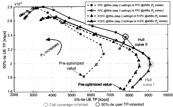
Fig. 7. 50%-ile user TP vs. 5%-ile user TP for FPC and FCPC.
