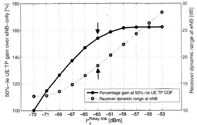
Fig. 13. 50%-ile user TP gain w.r.t. eNB-only deployment and eNB receiver dynamic range vs. P_0^{\text{Relaylink}} (with trade-off setting).
