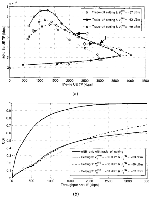
Fig. 12. (a) 5%-ile user TP vs. 50%-ile user TP for different values P_0^{\text{RN}} in relay deployment. Three settings can be noticed and (b) UE TP CDFs for these settings.
