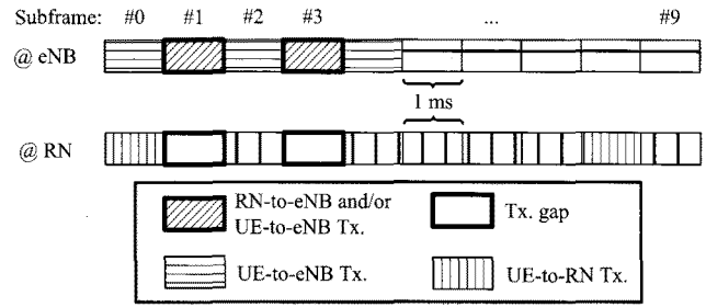
Fig. 2. FDD LTE-Advanced frame structure considering type 1 RNs. Transmission is abbreviated by Tx.
