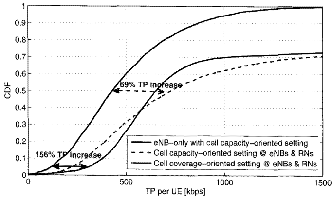
Fig. 5. CDF of TP per UE for common settings at eNBs and RNs. These simulation results show the explicit performance of type 1b RNs. The two lowermost CDF curves go to one at very high TP levels.
