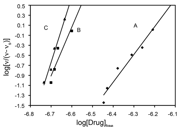
Figure 7. Hill plot for binding of drug to BSA in 0.01, 0.02 and 0.1% of protein: (A) n_H = 5.30 , \log K = 6.21 for 0.02%; (B) n_H = 9.70 , \log K = 6.60 for 0.1%; (C) n_H = 13.04 , \log K = 6.65 for 0.01%.
