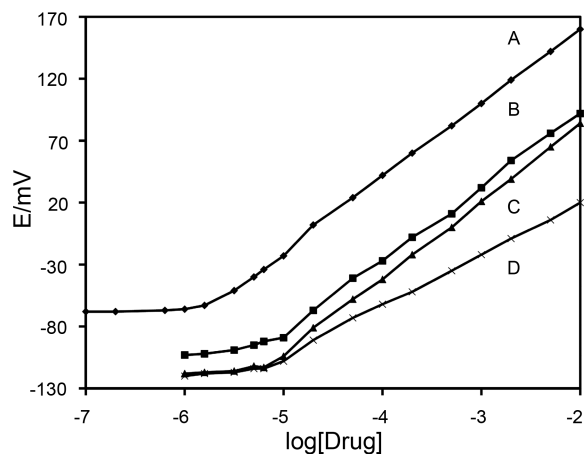
Figure 5. E.m.f. response of the ion selective electrode for dibucaine in various concentration of BSA: (A) 0; (B) 0.01; (C) 0.020; and (D) 0.10%.
