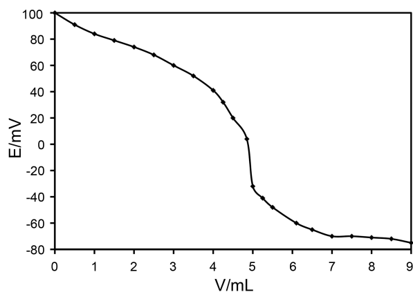
Figure 4. Potentiometric titration of dibucaine hydrochloride solution with NaTPB solution. Typical results for the titration of a 50.0 mL 1.0 \times 10^{-3} M dibucaine hydrochloride solution with 1.0 \times 10^{-2} M NaTPB.
