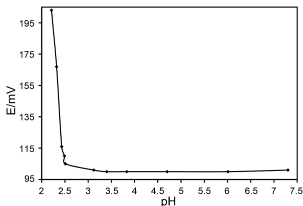
Figure 1. Influence of pH on the response of the membrane ( 1.0 \times 10^{-3} mol L -1 dibucaine).
