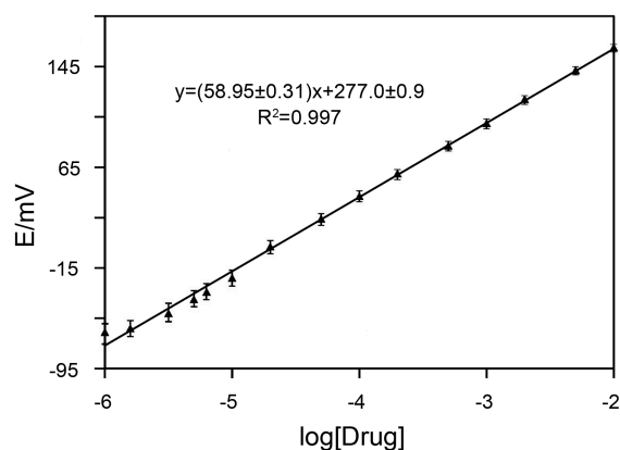
Figure 3. Calibration graphs of the membrane for dibucaine under the optimum conditions (each point was measured three times).
