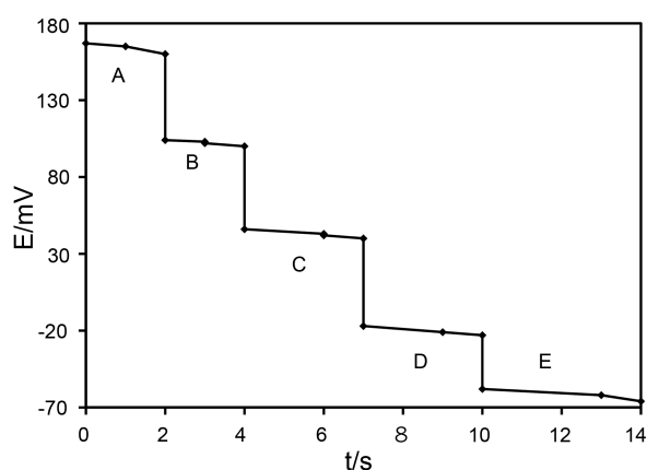
Figure 2. Response time of the electrode. (A) 1.0 \times 10^{-2} , (B) 1.0 \times 10^{-3} , (C) 1.0 \times 10^{-4} , (D) 1.0 \times 10^{-5} , and (E) 1.0 \times 10^{-6} dibucaine.
