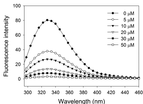
Figure 3. Fluorescence spectra of PPAR \gamma with 0-50 \mu M of biapigenin.
