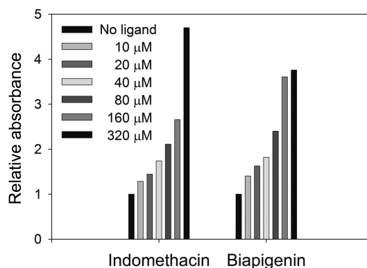
Figure 4. ELISA-based hPPAR \gamma activation assay with biapigenin and a positive control, indomethacin. hPPAR \gamma activation with ligand at a concentration range from 0 to 320 \mu M.
