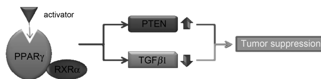
Figure 1. Schematic diagram of the mechanism of tumor suppression by PPAR \gamma .
