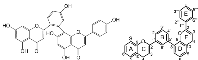
Figure 2. 2D structure of biapigenin.
